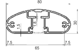
■ 7800 Elips Cam Profili 1,221 kg/m
